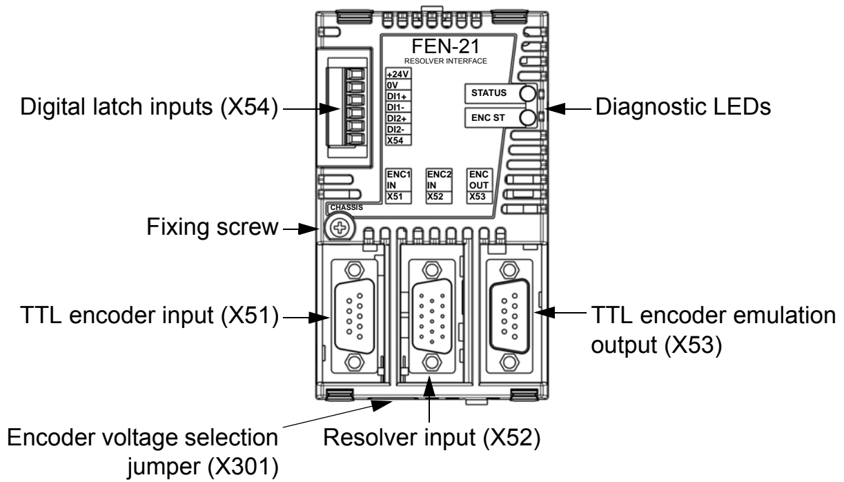
FEN-21 layout
