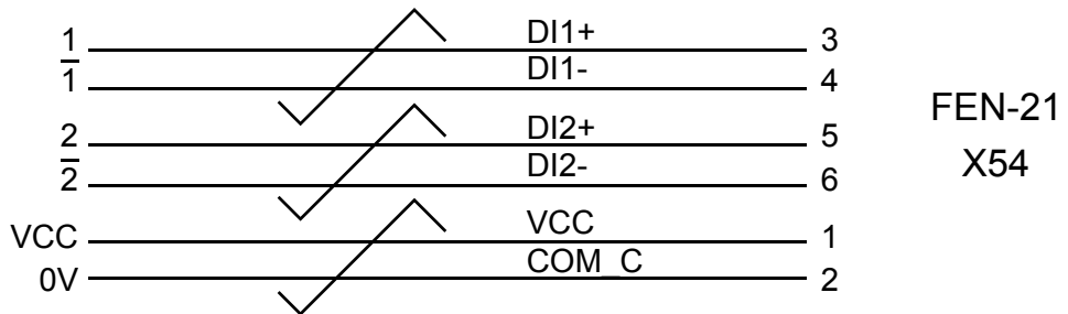
Digital inputs for position latching (X54)
